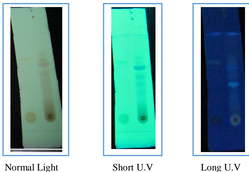
Figure 2: Thin layer chromatography of extract and standard (Quercetin)
