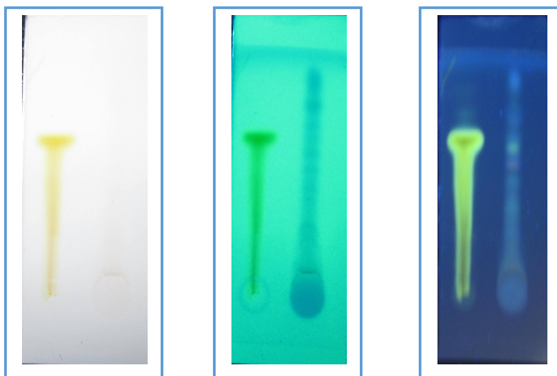
Figure 1: Thin layer chromatography of extract and standard (Gallic acid)
